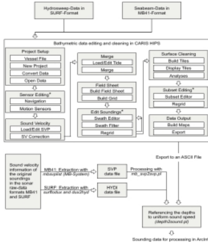
Figure 7-6. Final post-processing at the AWI with CARIS/HIPS
