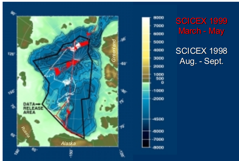
Figure 6-1. Track maps for the 1998 and 1999 SCIENCE ICe EXERCISES (SCICEX) surveys of the Arctic Basin. The terrain model for this slide was generated from the ETOPO-5 digital elevation dataset. Dark green and brown areas represent continents (Alaska, Russia and Greenland are labeled for reference). Light greens represent regions of shallow water depth; blues correspond to regions with water depths greater than 1000 meters and become darker with increasing depth. Contours are included for water depths of 1000, 2000, 3000, 3500, 4000, 4500, 5000 and 5500 meters. The thick black line around the margins of the Arctic Basin indicates the Data Release Area (labeled) in which the unclassified SCICEX data could be collected.
