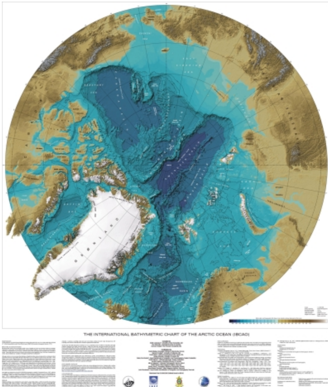
Figure 2-1. Draft of the proposed IBCAO replacement for GEBCO Sheet 5.17, to be printed at a scale of 1:6,000,000.
