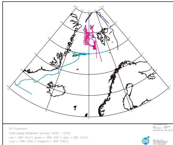
Figure 7-1. AWI 2001-2002 tracklines, Fram Strait
