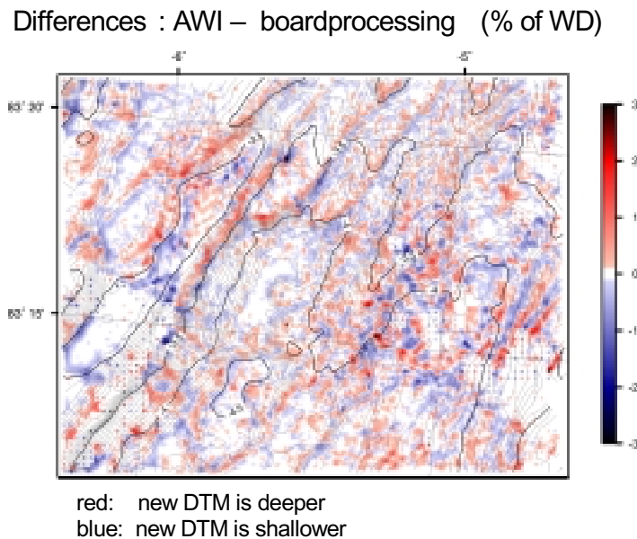
Figure 7-8. Difference between on-board processing and post-processing with HIPS. Contour lines determined after final post-processing
