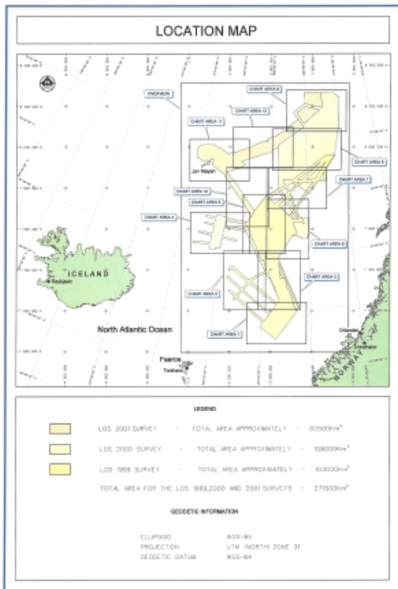
Figure 8-1. Surveys undertaken on behalf of the Norwegian Petroleum Directorate, for determining the outer limit of the juridical continental shelf.
