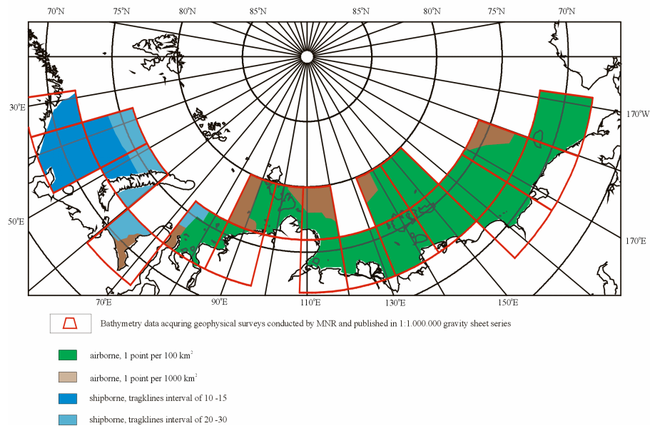
Figure 3-1. Bathymetric coverage of the Russian Arctic shelf.
