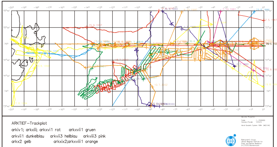
Figure 7-3. AWI tracklines over the continental slope of East Greenland
