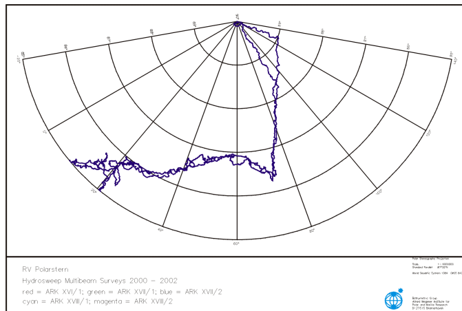
Figure 7-2. AWI 2002-2002 tracklines, Gakkel Ridge
