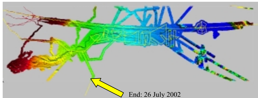
Figure 7-4. Present status of bathymetric mapping in the ARKTIEF-project. Track lines of “Polarstern”-leg ARK XVIII/1 (yellow) from 09 July until 26 July 2002
