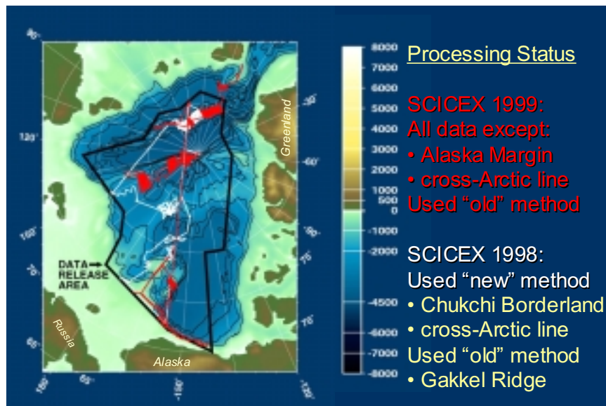
Figure 6-4. Current status of SCICEX processing.
