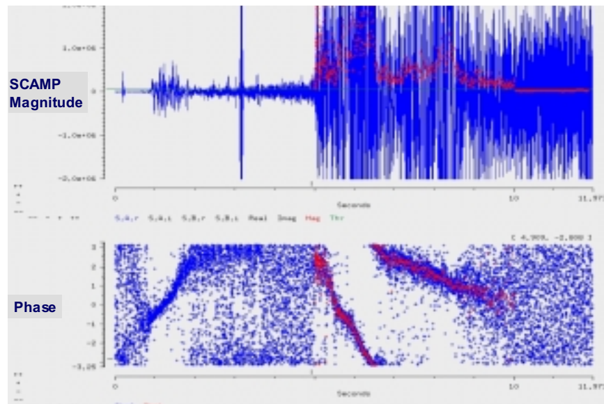
Figure 6-2. Raw SCAMP acoustic data are typically examined as magnitude and phase values (although, as can be seen on the labels near the center line of this figure, it is also possible to examine the real and imaginary components of the synthesized row A and row B data. (The SCAMP SSBS actually has four transducer rows, but these are electronically synthesized to yield two virtual rows of information).
