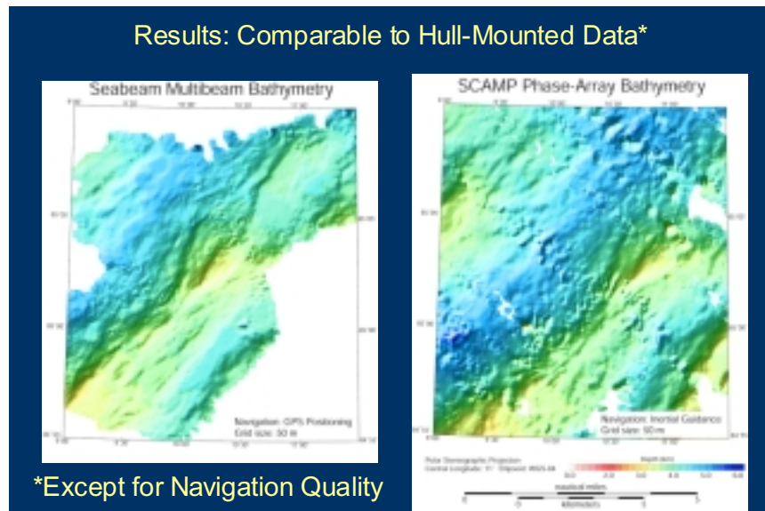
Figure 6-3. Comparison of bathymetry data collected by the USCGC Healy using the hull-mounted Seabeam 2112 system (left) and SCICEX bathymetry for the same region collected by the Seafloor Characterization and Mapping Pods (SCAMP; right). In this figure both datasets are gridded at the same grid cell size (50 m).
