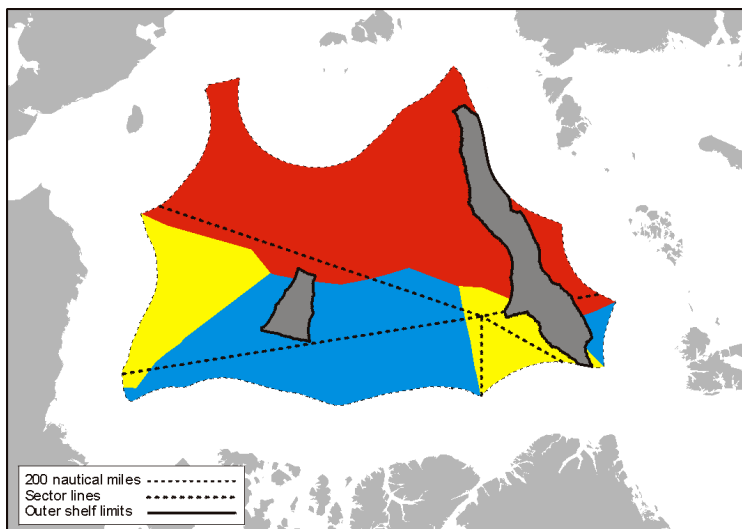
Figure 15-3. The colour portions of the figure above illustrate the continental shelf partitions that could result if all five coastal states agreed to the equidistance principle. For comparison, the boundaries constructed according to the sector principle are shown with dashed lines.
